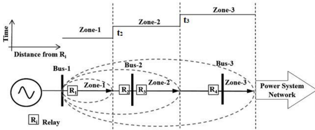
Fig. 2. Zones of the distance relay
