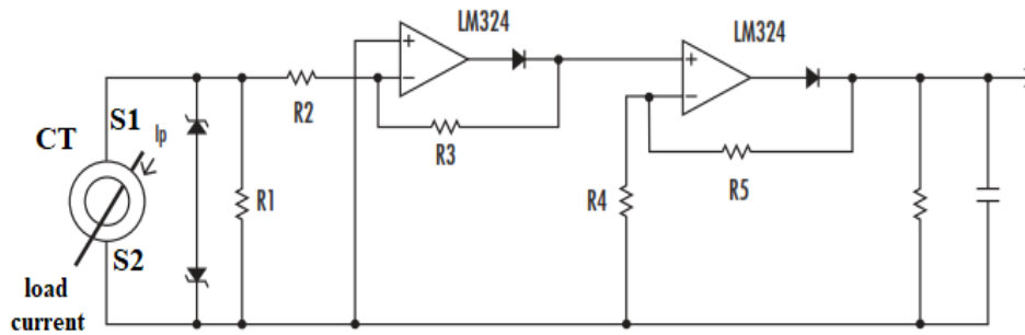
Fig. 4. Signal conditioning circuit for CT
