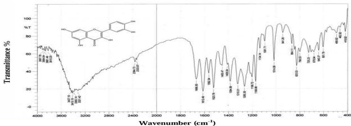
Figure 1: The IR spectrum of quercetin
